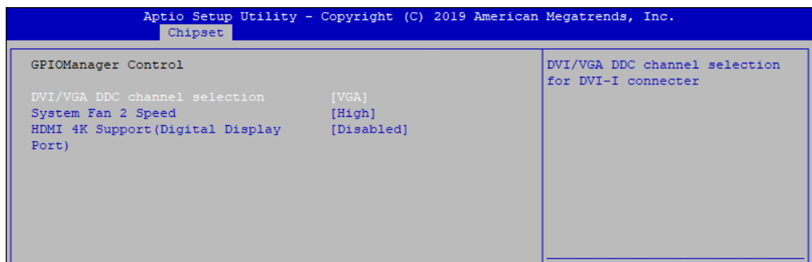
Figure 4-4-3 : GPIOManager Configuration
