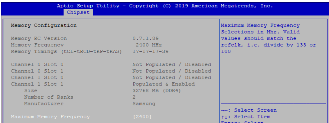
Figure 4-4-1-1 : Memory Information
