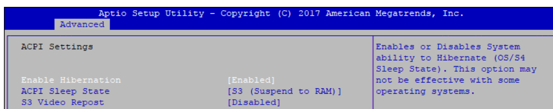
Figure 4-3-5 : ACPI Settings
