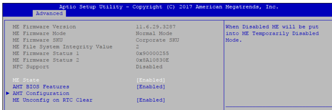
Figure 4-3-3 : PCH-FW Settings
