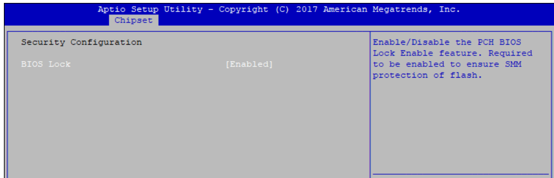
Figure 4-4-2-3 : Security Settings
