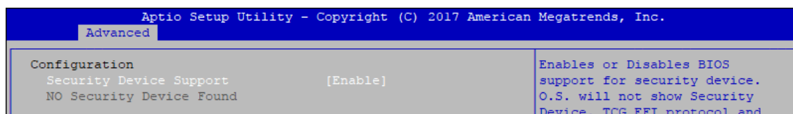
Figure 4-3-4 : Trusted Computing
