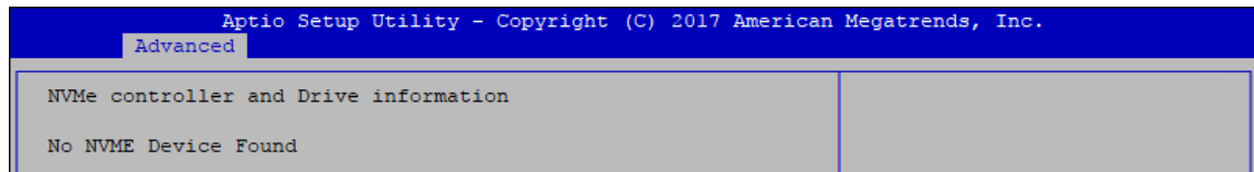
Figure 4-3-15 : NVMe Settings
